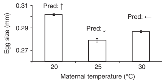
Fig. 4. Effect of temperature on the mean ( \pm s.e.) size of eggs that D. rerio mothers produced. Arrows indicate prediction of optimality model based on our findings from experiment 1. Up arrow indicates maternal fitness is predicted to be maximised by producing the largest offspring size, down arrow indicates maternal fitness is predicted to be maximised by producing the smallest offspring and sideways arrow indicates maternal fitness is predicted to be maximised by producing offspring of intermediate size.
