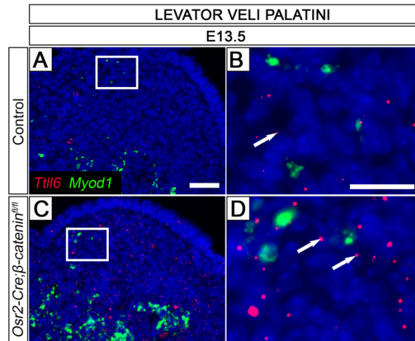
Fig. S1. Loss of Wnt signaling in mesenchymal cells leads to an increase of Till6 expression. (A-D) Till6 (red) and Myod1 (green) in situ RNAScope hybridization in control (A-B) and Osr2-Cre;β-catenin fl/fl mice (C-D). Boxes in A and C show approximate location of images in B and D. White arrows in B and D point to positive signals. Scale bar in A indicates 50 μm in A, and C; scale bar in B indicates 20 μm in B and D.
