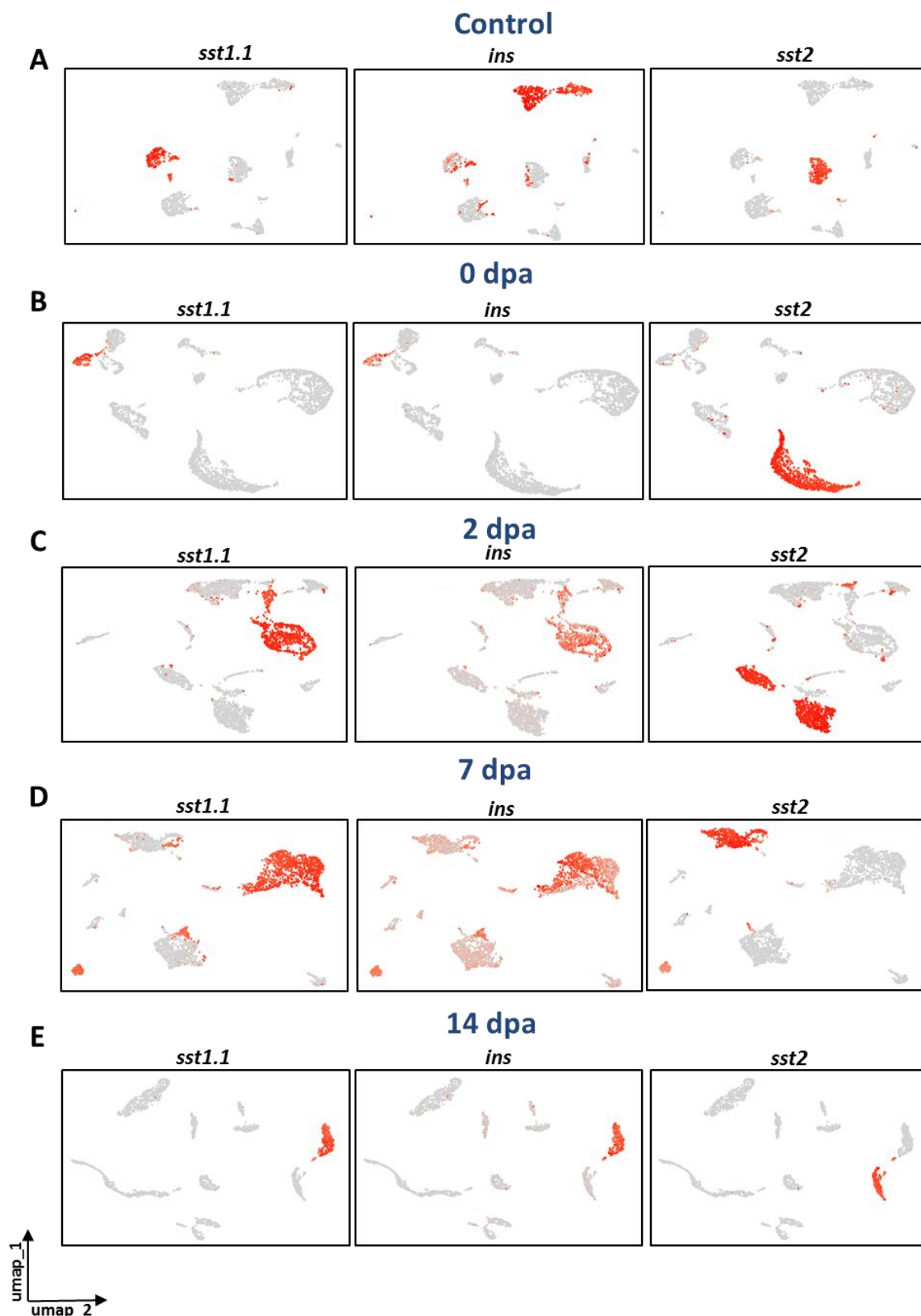
Fig. S6. \delta 1 - but not \delta 2 -cells express insulin upon \beta -cell loss in adults. (A-E) UMAP plot representation of adult zebrafish pancreatic cells showing expression of ins , sst1.1 , and sst2 at various \beta -cell regeneration time-points: Control, 0 dpa, 2 dpa, 7 dpa, and 14 dpa.
