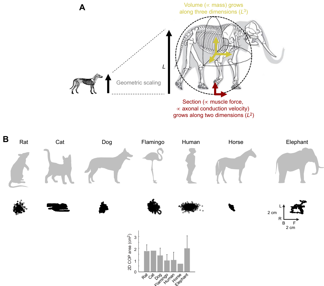
Fig. 3. Scaling of postural control in terrestrial mammals. (A) Differences imposed by scaling between dogs and elephants. L , length. (B) COP excursion area during quiet standing is similar across species of different sizes. Example COP traces were digitized and redrawn from Funato et al. (2017) (rat), MacPherson and Horak (2012) (cat), Chang and Ting (2017) (flamingo), Ivanenko et al. (1999) (human) and Clayton and Nauwelaerts (2014) (horse). The COP excursion areas were also computed when raw data were available. If not (for cats and horses), the COP excursion areas were estimated based on the reported COP displacement (Clayton and Nauwelaerts, 2014; MacPherson and Horak, 2012).
