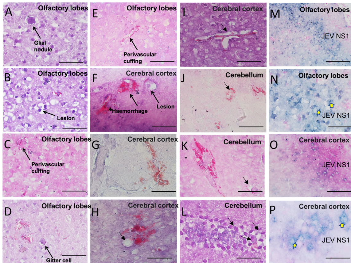
Fig. 4. Pathology of JEV in C57BL/6 mouse model. Representative Haematoxylin and Eosin-stained slices of brain tissue at 40× magnification (20× magnification in M and O) represent histopathology of brain from C57BL/6 (3-4 weeks old, n=3 ) mice infected with 100 \mu l JEV-S3 ( 10^7 pfu) through the IP route. (A-E) Glial nodule, necrotic lesions and perivascular cuffing are the histologic features demonstrated in the olfactory lobes of JEV-infected brain. (F-L) Perivascular haemorrhage, necrotic lesion and infiltrating cells in the cerebral cortex and cerebellum. Arrow in H indicates a lesion; arrows in L indicate immune cell infiltration. (M-P) Immunoperoxidase staining with Haematoxylin counterstain showed the presence of viral antigens (NS1) in olfactory lobes and cortex. Scale bars: 5 \mu m.
