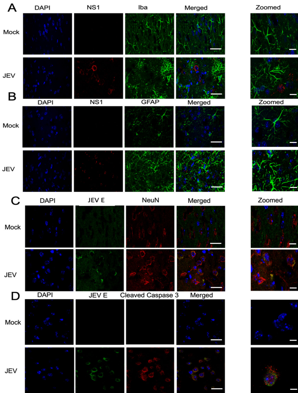
Fig. 5. Microglia, astrocyte and caspase activation in JEV-infected mouse brain. C57BL/6 (3-4 weeks old) mice ( n=3 ) were inoculated IP with 100 \mu l JEV-S3 ( 10^7 pfu), and brain tissues were harvested 24 h post-onset of symptoms. Microglia, astrocytes, neuron and activated caspase-3 were visualized by immunohistochemical staining of the brain sections from mock- and JEV-infected mice using antibodies against IBA1 (A), GFAP (B), NeuN (C) and (cleaved) caspase-3 (D). Viral infection in the brain tissue sections was demonstrated by staining for viral NS1 (A,B) and E (C,D) proteins. Nuclei were stained with DAPI (blue). Scale bars: 10 \mu m (5 \mu m in zoomed images).
