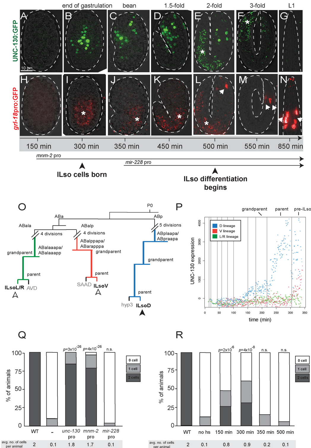
Fig. 3. UNC-130 is expressed in a restricted lineage before the onset of differentiation. (A-G) Time course of embryos expressing UNC-130:GFP. (H-N) Time course of embryos expressing grl-18pro :GFP (pseudo-colored red). Asterisks indicate gut autofluorescence. Arrows indicate grl-18+ ILso cells. (O) Lineage diagram of a subset of embryonic cell divisions derived from the AB blastomere that gives rise to ILsoD (blue), ILsoV (red) and ILsoL/R (green) glia. (P) Levels of UNC-130:GFP signal in ILsoD (blue), ILsoV (red) and ILsoL/R (green) lineages over developmental time. Vertical lines indicate cell divisions. Subtraction of background fluorescence signal results in negative values for some cells. (Q) Heterologous promoters were used to drive expression of unc-130 in the unc-130 mutant strain, and the extent of rescue was assessed. Timing of mnm-2pro and mir-228pro expression is marked in A. Percentage of animals expressing grl-18pro :YFP in zero, one or two ILsoD glia in each condition. Average number of cells marked per animal is listed under each condition. n=50 animals per condition. P -values were calculated by Fisher's Exact test. (R) unc-130 mutant embryos expressing hsp:unc-130 were heat shocked at different time points and the extent of rescue was assessed. Percentage of animals expressing grl-18pro :YFP in zero, one or two ILsoD glia in each condition. Average number of cells marked per animal is listed under each condition. n=50 animals per condition. P -values were calculated by Fisher's Exact test.
