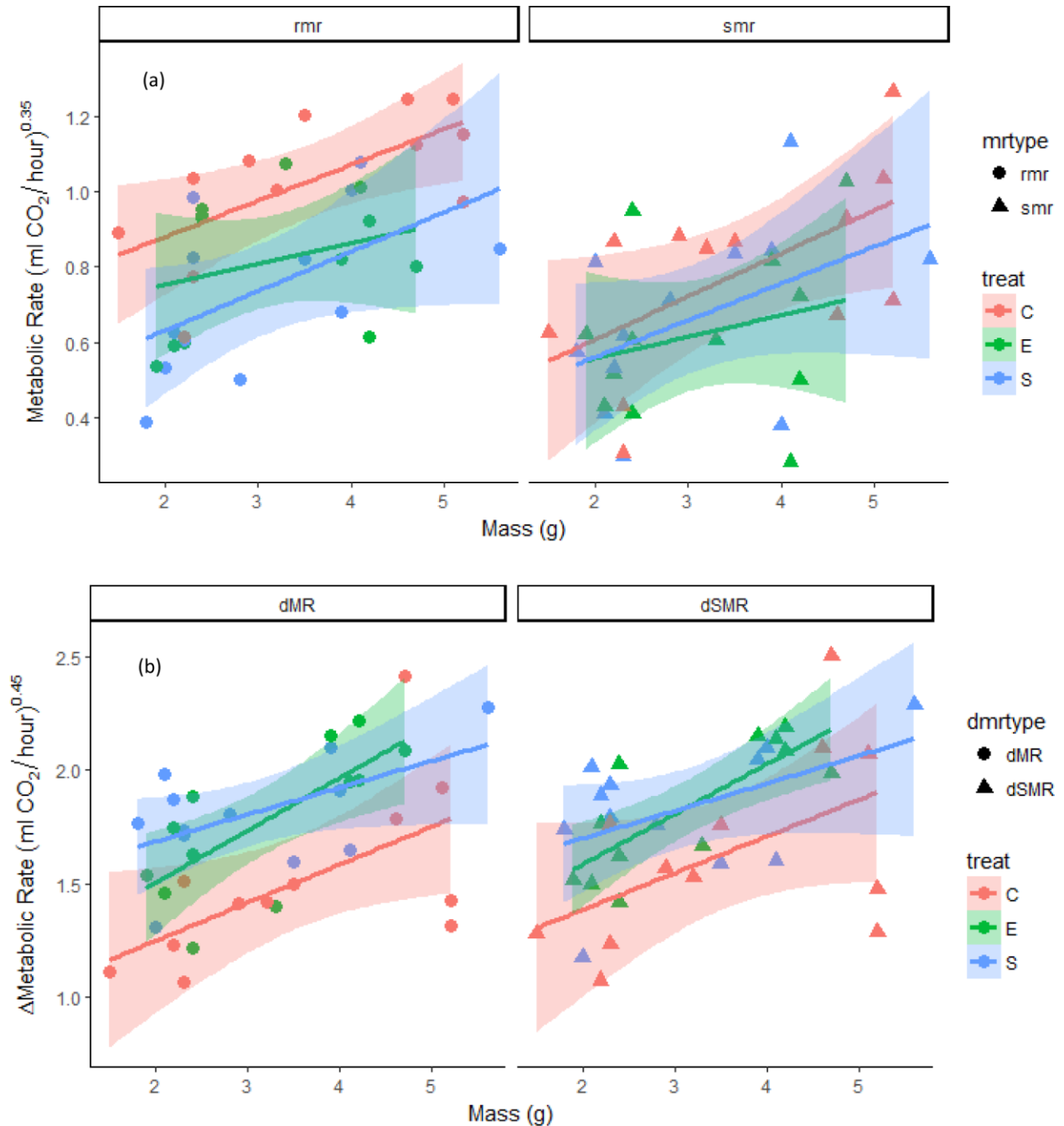
Fig. 1. Influence of mass, MR type, and training treatment on (a) MR^{0.35} and (b) (\Delta MR)^{0.45} . (a)
