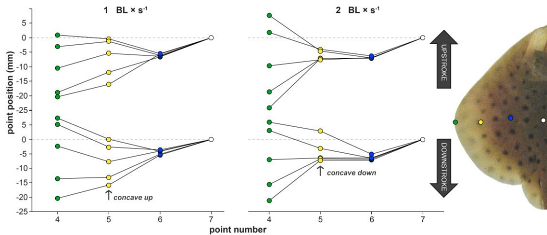
Figure 7. Pattern of chordwise curvature on the wing during locomotion. Fin conformation at the mid-disc mediolateral position (markers shown on the skate wing to the right) during upstroke and downstroke, at two speeds. Thick arrows indicate direction of movement. Curvature calculations from these data are discussed in the text. Note that during the later stages of the downstroke at 2 \text{ BL} \times \text{s}^{-1} , the wing is concave into the direction of motion, indicating active control of wing shape.
