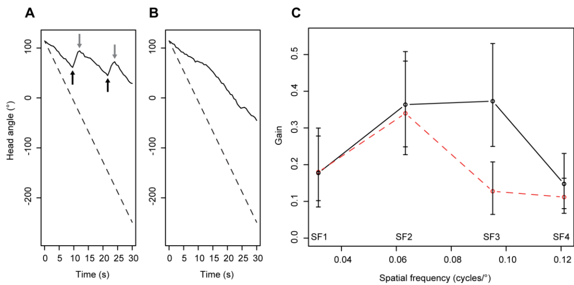
Fig. 1. Smooth and saccadic responses to moving square-wave gratings and averaged responses to gratings seen through the naturalistic horizontally or weakly vertically polarized light field. A: In a relatively small number of trials (see text) animals responded to the movement of the grating (indicated by the dashed line) with periods of smooth tracking followed by rapid, saccadic, movement of the head in the opposite direction (A; black arrows indicating start of saccade and grey arrows indicating start of smooth tracking). B: The majority of animals tracked the drum smoothly but, typically, lagged behind the movement of the drum, indicated by gain values < 1.0 in all cases. C: the responses (gain) of larvae to four spatial frequencies (SF1 to SF4; 0.032, 0.063, 0.095, 0.121 cycles per degree respectively) in horizontally polarized (black solid lines) and vertically polarized (red dashed lines) light fields. There was a significant difference in response to grating SF3 between the two light fields. Error bars represent \pm 1 standard deviation.
