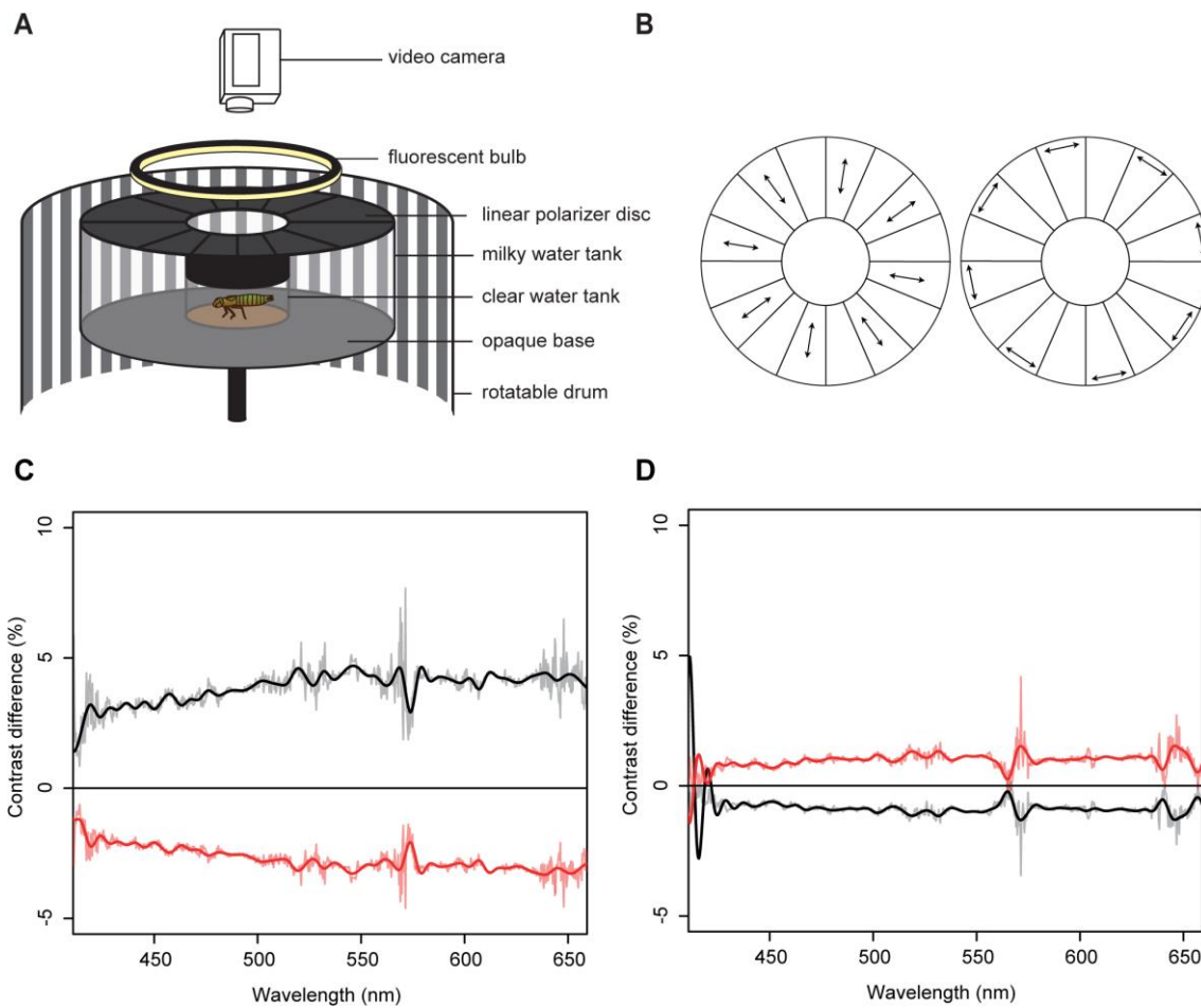
Fig. 4. Experimental apparatus used to test the optomotor response and the changes in contrast of the square-wave gratings when polarization filtering was applied. A: Experimental set up to test the optomotor response of dragonfly larvae to a moving square-wave grating of vertical stripes. The subject animal was contained in the stationary central cylinder of clear water, which was surrounded by a concentric outer tank containing dilute milk solution. Light to the latter, from above, was polarized by one of two linear polarizing discs (B), consisting of radially or tangentially orientated linear polarizers, resulting in vertically or horizontally polarized light (respectively) being scattered towards the subject. This veiling light field reduced the contrast of the grating, which was fixed to a rotatable outer drum. The animal's response was assessed by their measuring their ability to visually track the rotation of the grating. B: Polarizer discs used to change the polarization of the light illuminating the milky water tank, constructed of sectors of Polaroid™ filter. The arrows indicate the transmission axis of the linear polarizer in each sector. Two light fields were created using these discs independently: one vertically polarized (left disc), and the other horizontally polarized (right disc). C and D: Change in intensity contrast of the grating stripes, from measurements made without a linear polarizer, when measurements were made
