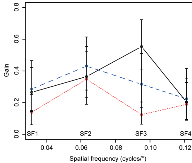
Fig. 2. Averaged responses to different grating contrasts. Responses (gain) of larvae to gratings having four different spatial frequencies (SF1 – SF4; 0.032, 0.063, 0.095, 0.121 cycles per degree, respectively) and three different intensity contrasts, 16.3% (red dotted lines), 20.3% (blue dashed lines) and 24.3% (black solid lines), seen through a vertically polarized light field. Error bars represent \pm 1 standard deviation. Responses varied most to grating SF3, with gain increasing with grating contrast.
