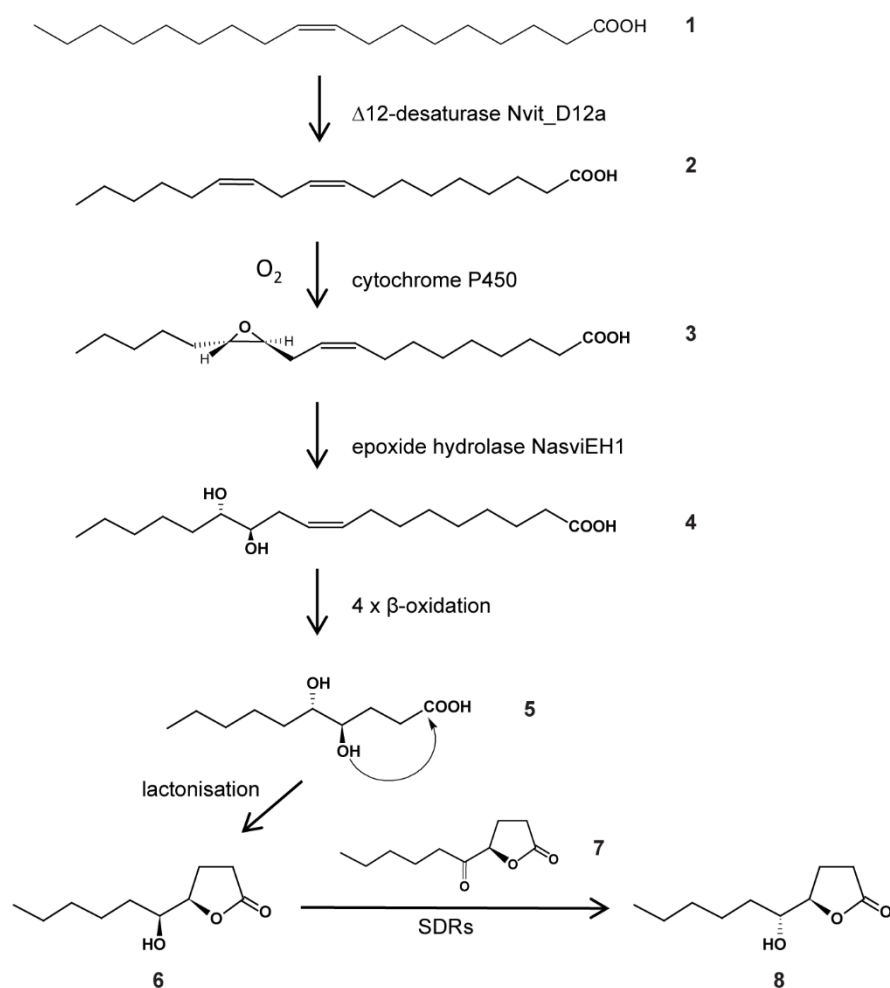
Figure 1. Biosynthetic pathway of the N. vitripennis sex pheromone components. Biosynthesis starts from oleic acid (1, C18:1 Δ9 ) (Blaul et al., 2011) which is converted by the \Delta -12-desaturase Nvit_D12a to linoleic acid (2, C18:2 Δ9,12 ) (this study and Blaul et al., 2014). C18:2 Δ9,12 is epoxidised by a hitherto uncharacterised cytochrome P450 enzyme. The resulting 12,13-epoxy-octadec-9Z-enoic acid (3), is hydrolysed by the epoxide hydrolase NasviEH1 (Abdel-latif et al., 2008) to (12R,13S)-12,13-dihydroxy-octadec-9Z-enoic acid (4); chain shortening by four steps of \beta -oxidation leads to (4R,5S)-4,5-dihydroxydecanoic acid (5) which lactonises to (4R,5S)-5-hydroxy-4-decanolide (6). Epimerisation of (6) by the short chain dehydrogenases/reductases (SDRs) NV10127, NV10128 and NV10129 with (4R)-5-oxodecanolide (7) occurring as an intermediate, finally leads to (4R,5R)-5-hydroxy-4-decanolide (8) (Niehuis et al., 2013, Ruther et al., 2016).
