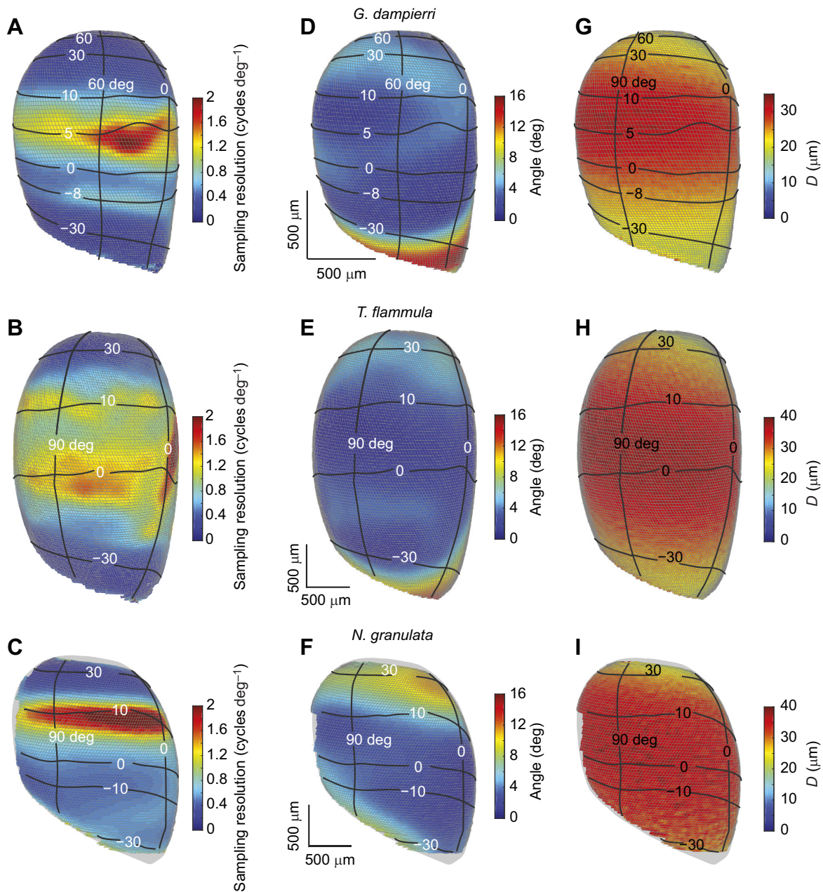
Fig. 6. Resolution, direction of ommatidia in relation to local eye curvature, and facet size. (A–C) Back projections of vertical sampling resolution on the eyes of (A) G. dampieri , (B) T. flammula and (C) N. granulata showing the location of the ommatidia that form the visual streak on the eye. (D–F) The angular differences between the ommatidial axes and the local surface normal indicate that in all three animals the visual streaks are located in the flat part of the eye where the ommatidial axes are closely aligned with the local surface normal (<3 deg). (G–I) The biggest facets are located at approximately 5 deg above the horizon in the lateral part of the eye, approximately in the middle of the elongated eye space. The grey surface underneath the map of N. granulata shows the complete outline of the eye.
