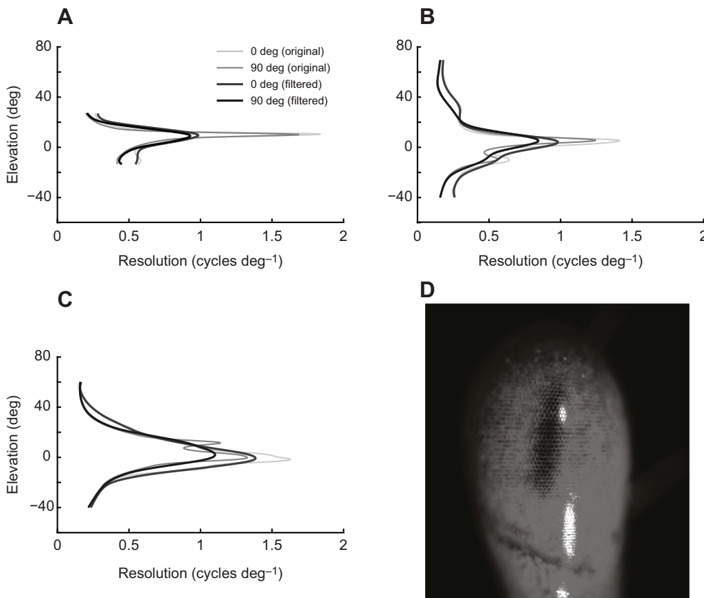
Fig. 8. Spatial averaging in the pseudopupil method. The vertical sampling resolution of (A) N. granulata , (B) G. dampieri and (C) T. flammula filtered with an averaging window of 10 deg. This averaging, which resembles the typical 10–20 deg averaging of visual space by the pseudopupil method, diminishes the secondary visual streak in both species of fiddler crabs and results in a wider and shorter visual streak compared with the results obtained via the current method. (D) Image of the pseudopupil of a G. dampieri taken in the same optical set-up used by Smolka and Hemmi (2009), which employed a microscope with a numerical aperture of 0.1. The pseudopupil image is composed of approximately 85 ommatidia and has an indistinct boundary. The centre of the pseudopupil needs to be defined, and located, in order to map its position across the eye.
