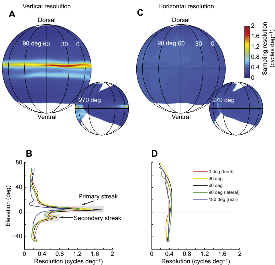
Fig. 4. Variation of vertical and horizontal sampling resolution in a male G. dampieri . (A,B) Vertical and (C,D) horizontal sampling resolution on spherical maps (A,C) and vertical transects (B,D). The horizontal resolution remains fairly even across the eye. The two distinct visual streaks of vertical resolution are located at 5 deg (primary streak) and -8 deg (secondary streak) of elevation.
