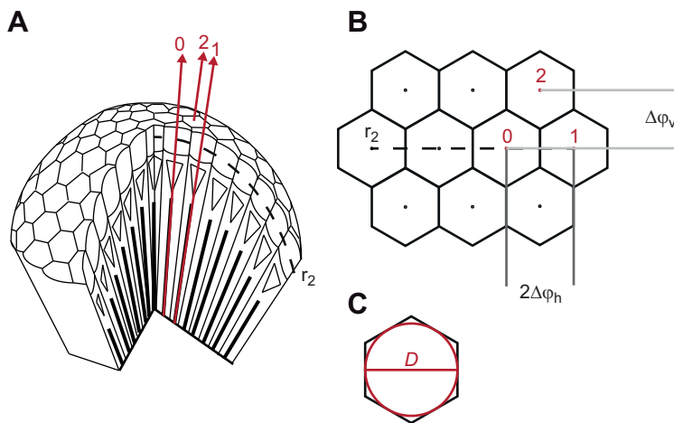
Fig. 2. Calculation of interommatidial angles and facet diameter.
