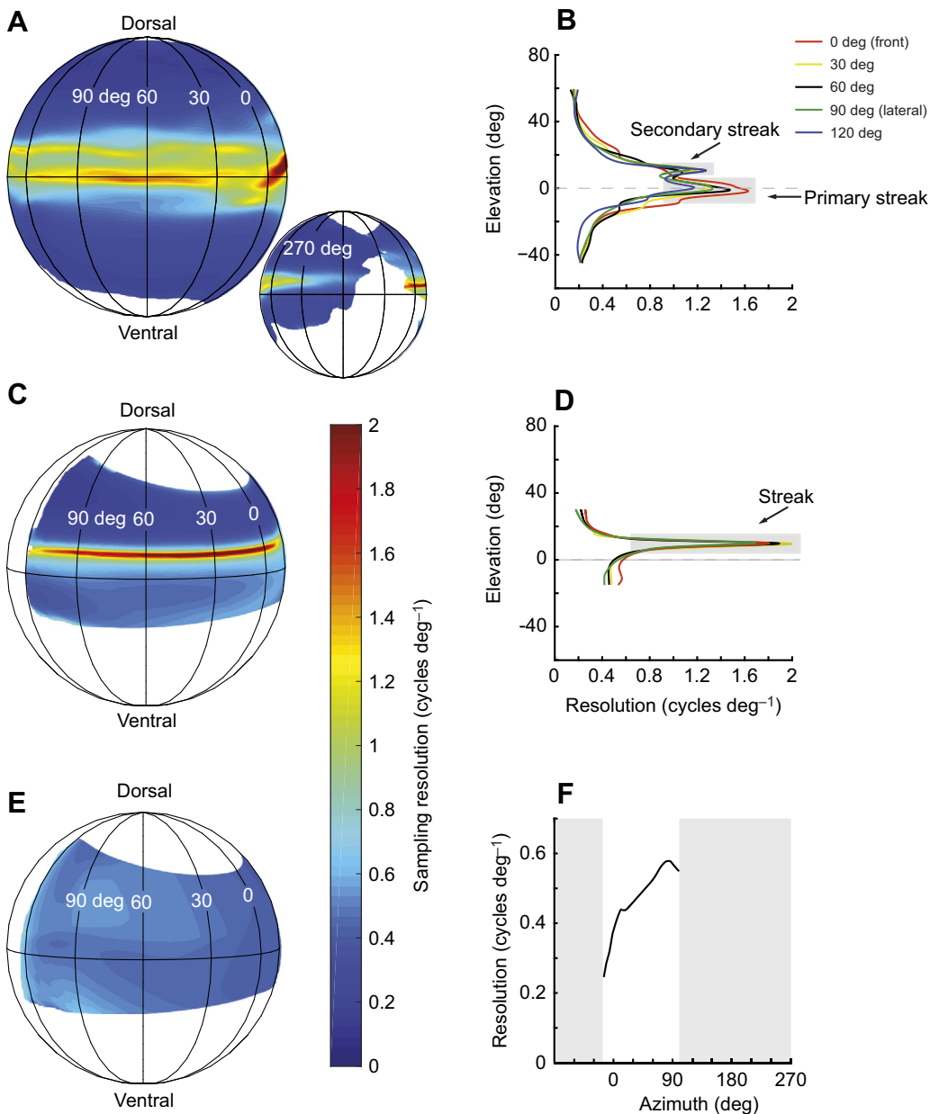
Fig. 5. Sampling resolution in Tubuca flammula and Neohelice granulata . (A) The spherical map and (B) vertical transects of vertical sampling resolution clearly show two visual streaks in T. flammula . In contrast to G. dampieri , the primary streak is found at a lower elevation (0 deg) compared with the secondary streak, which is found more dorsally (at 10 deg of elevation). (C) Vertical sampling resolution and (D) vertical transects in N. granulata show the presence of only one visual streak at 10 deg above the horizon. (E) The horizontal resolution of N. granulata is not uniform and increases towards the lateral part of the eye. (F) A horizontal transect of horizontal resolution at 10 deg of elevation in N. granulata . Shaded area indicates no data available.
