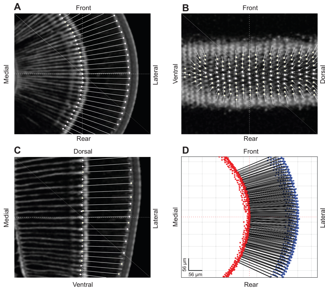
Fig. 1. 2D and 3D reconstructions of the ommatidial axes of Gelasimus dampieri . (A–C) The centres of each cornea and the tip of the corresponding rhabdoms (shown by points) were labelled by viewing micro-computed tomography (microCT) images of compound eyes in three perpendicular planes. The two corresponding points identify the optical axis of the crystalline cones (solid lines). (A) Horizontal plane (perpendicular to the eye stalk, approximately through the middle of the eye). (B,C) Vertical planes through the mid-point in A as marked by the dotted crosshairs. B shows the tip of rhabdoms and the base of the crystalline cones and shows how the axes of these lenses diverge along the horizontal direction. (D) The coordinates of the centres of the corneas (blue points), rhabdoms (red points) of the ommatidia visible in A (and their neighbours), and the optical axes of ommatidia, as calculated based on these points in 3D space.
