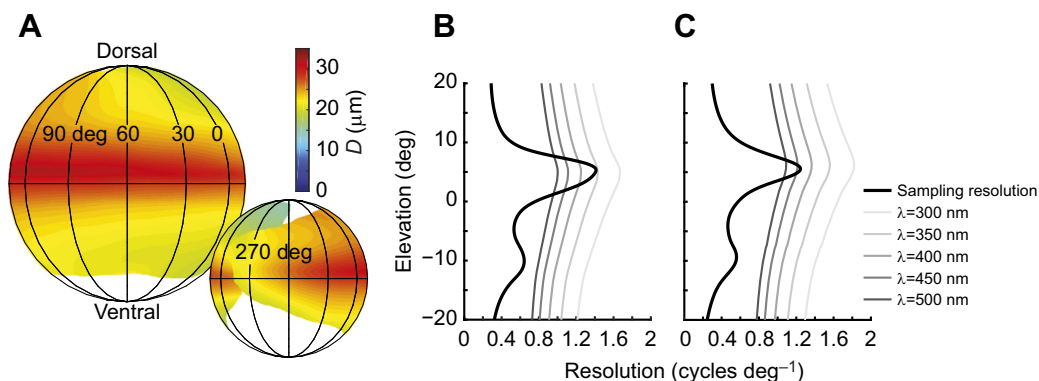
Fig. 7. Facet diameter and optical resolution in the male G. dampieri . (A) The variation of facet diameter projected onto a surrounding sphere. The facets looking in directions -5 to 20 deg in elevation are larger. (B,C) Comparison of vertical sampling resolution (black lines) estimated from interommatidial angles, and optical resolution (grey lines) estimated from the diameter of the Airy disk images produced by ommatidial facets and lenses, in (B) frontal and (C) lateral vertical transects of the eye. Optical resolution depends on the wavelength of sampled light and is shown for five different wavelengths. Direct comparison of sampling versus optical resolution suggests that the lateral region is able to resolve spatial patterns of longer wavelength than the frontal visual field.
