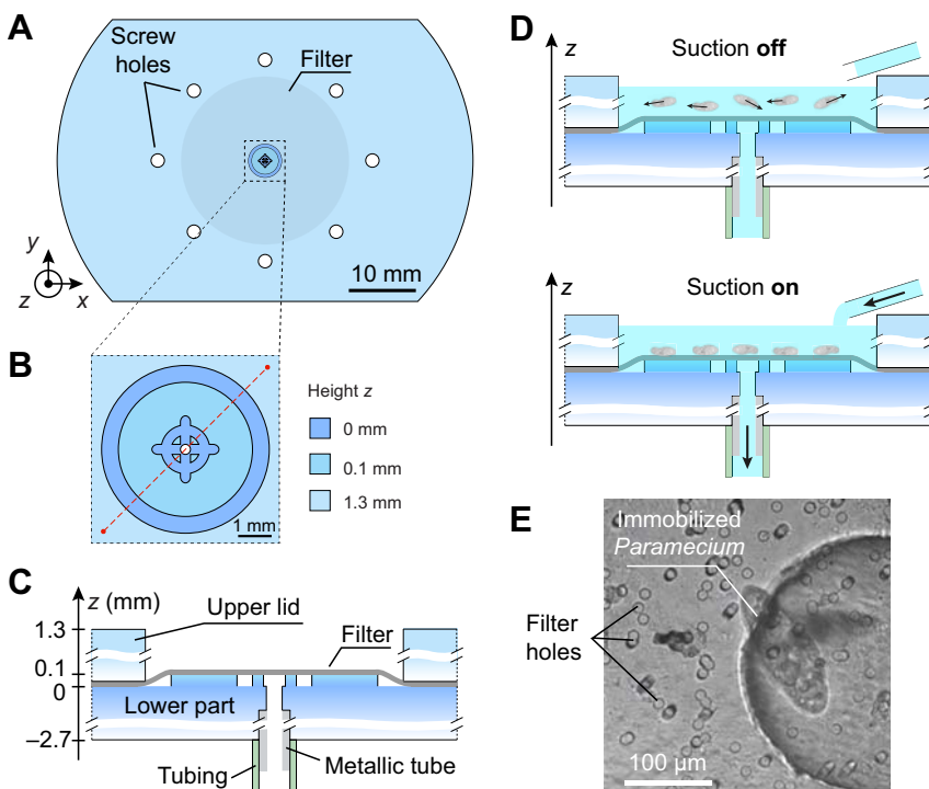
Fig. 1. Diagram of the immobilization device. (A) Top view of the device. The filter (shaded grey disk) is sandwiched between an upper lid and a lower part all made of Plexiglas, tightened together with 8 screws. (B) Close-up of the centred microfluidic mesa-like structure. The z=0 height origin is arbitrarily taken at the base of the mesa-like structure. (C) Lateral view along the red dashed line in B. (D) Principle of the immobilization process. Without suction (upper panel), ciliates in the centred pool swim freely. Once suction is switched on (lower panel), ciliates are immobilized against the filter. Their bathing liquid is pumped using either a peristaltic pump or a depression tank. The liquid is reinjected (when using the pump) or supplemented (when using the depression tank) in the pool to maintain the level of the bath constant. (E) Bright-field image of a single Paramecium immobilized with the current device (top view). The round object is a microfluidic channel below the filter, the left end of the cross in B.
