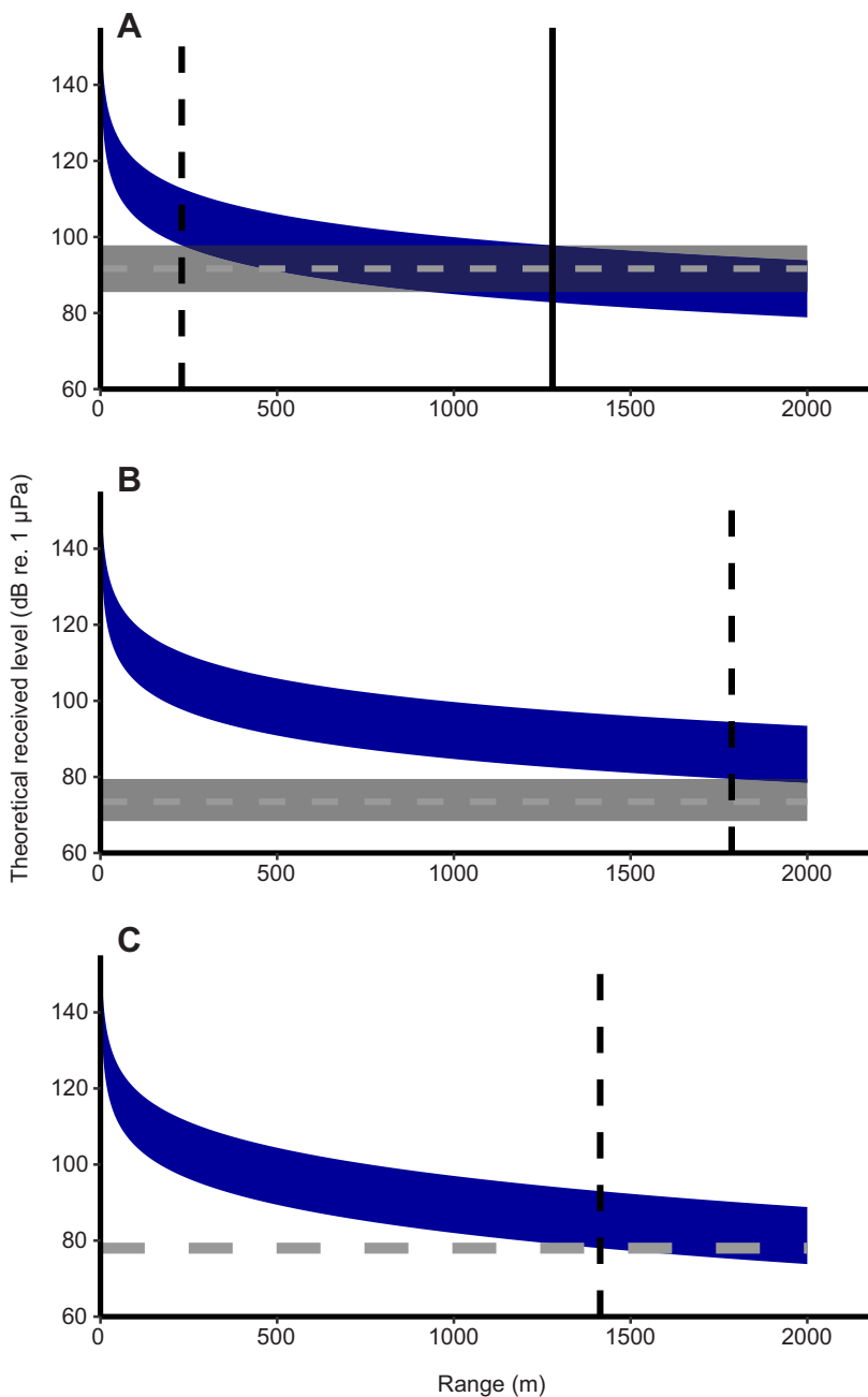
Fig. 3. Sound propagation modelling for a pure tone (dark blue) over a range of 2000 m. (A) 1 kHz, (B) 5 kHz and (C) 20 kHz pure tone with source level of 145–160 dB. Medians with 25 and 75 percentile detection thresholds (A and B, grey dashed line and grey shaded area, respectively) and Wenz ambient noise level (C, grey dashed line) influenced signal detection at frequency-specific distances. Signals with a low source level dropped below the maximum detection threshold at some point for all frequencies (vertical dashed black lines). For 1 kHz signals, signals with a high source level also dropped below the detection threshold at 1279 m (vertical solid black line).
