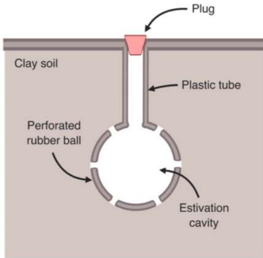
Figure S1: Schematic representation of the artificial estivation burrow used for pO_2 measurements.
