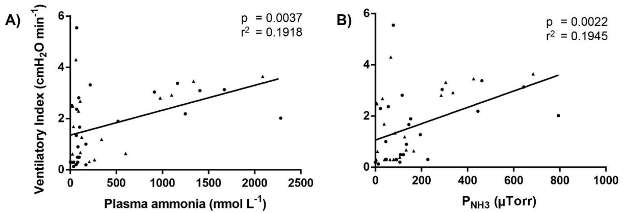
Figure S4. Correlation of ventilatory index with (A) total plasma ammonia concentration ( T_{\text{Amm}} ) and (B) gaseous ammonia tension ( P_{\text{NH}_3} ) in individual hagfish injected at a dose of 1,000 \mu\text{mol kg}^{-1} or 70 \mu\text{mol kg}^{-1} of ammonium salts ( \text{NH}_4\text{HCO}_3 and \text{NH}_4\text{Cl} ) in Series IV. The significance ( p ) and r^2 values are shown.
