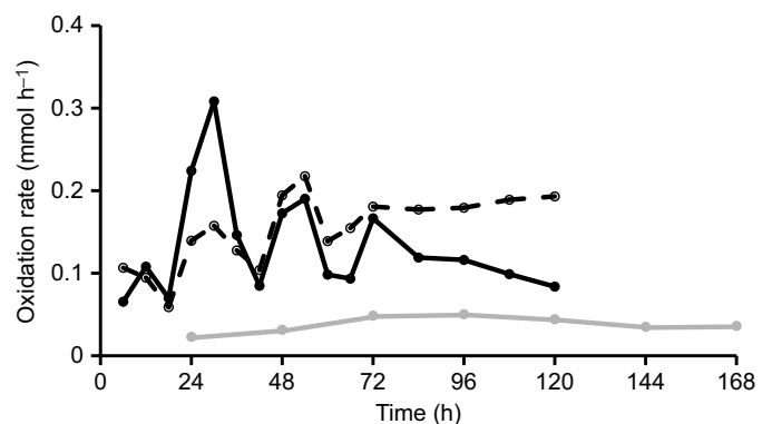
Fig. 3. Mean oxidation rates of palmitic acid in A. atra across temperatures. Grey dots and line indicate the rate of 13 C-palmitic-acid oxidation at 20°C, white circles and dashed line at 25°C, and solid line at 32°C.
