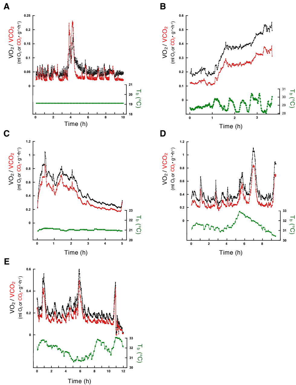
Fig. S3. Additional examples of physiological disconnects in tenrecs. Note the numerous instances where VO 2 /VCO 2 is changing without a concomitant change to T b (A, B, C), or where T b is changing without the expected change in VO 2 /VCO 2 (D and E). Additionally, these physiological disconnects are sustained over the course of hours in most instances.
