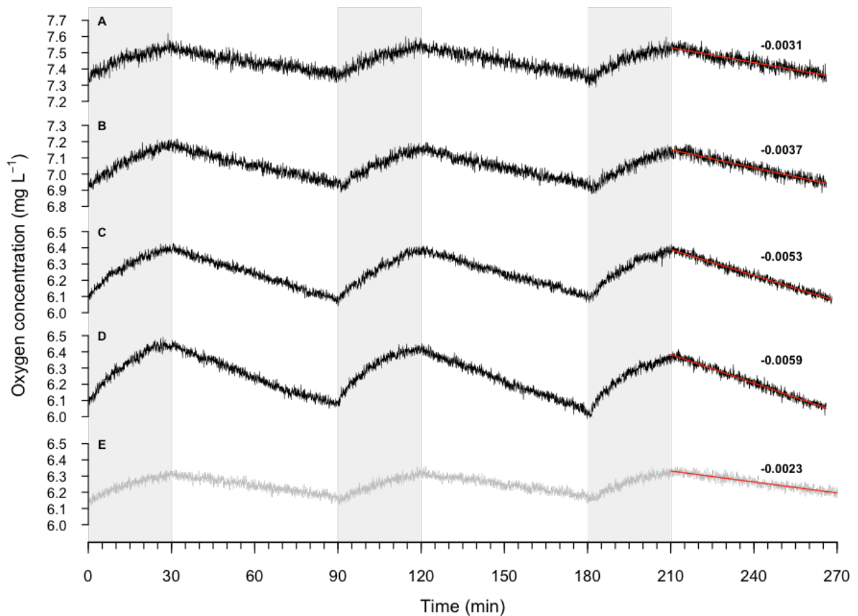
Figure S2. Raw oxygen traces for a representative sea snake illustrating the cutaneous oxygen consumption ( \dot{V}O_{2\text{cut}} ) at four temperature treatments (A) 21°, (B) 24°, (C) 27° and (D) 30°C. Background (microbial) respiration was measured at all temperatures and subtracted from sea snake \dot{V}O_{2\text{cut}} ; a representative background trace at 30°C is presented (E). Grey shading represents periods when flush pumps were running. Red lines represent the measurements of change in oxygen concentration ( \Delta cO_2 ) measured during sealed cycles ( \Delta t ), as in equation 1 of the main text.
