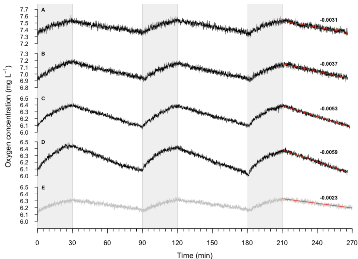
Figure S2. Raw oxygen traces for a representative sea snake illustrating the cutaneous oxygen consumption ( \dot{V}O_{2cut} ) at four temperature treatments (A) 21°, (B) 24°, (C) 27° and (D) 30°C. Background (microbial) respiration was measured at all temperatures and subtracted from sea snake \dot{V}O_{2cut} ; a representative background trace at 30°C is presented (E). Grey shading represents periods when flush pumps were running. Red lines represent the measurements of change in oxygen concentration ( \Delta cO_2 ) measured during sealed cycles ( \Delta t ), as in equation 1 of the main text.
