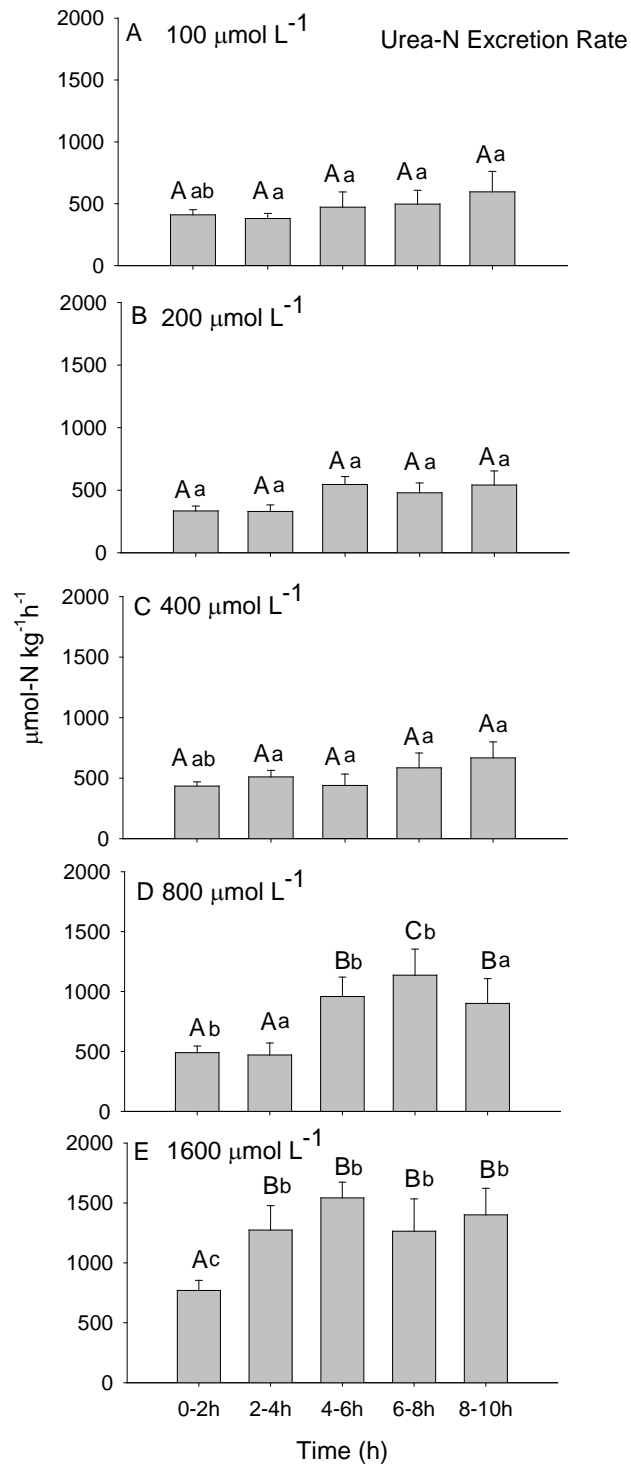
Fig. S2. Urea-N excretion rates of dogfish sharks over successive 2-h periods during 10-h exposures to nominal starting seawater ammonia-N concentrations of (A) 100; (B) 200; (C) 400; (D) 800; and (E) 1600 µmol L -1 . Means ± 1 SEM (N = 10). Means sharing the same upper case letter do not differ significantly (repeated measures ANOVA, followed by the Holm-Sidaktest, P > 0.05) among time periods within a concentration. Means sharing the same lower case letter do not differ significantly (P > 0.05) among concentrations within a time period.
