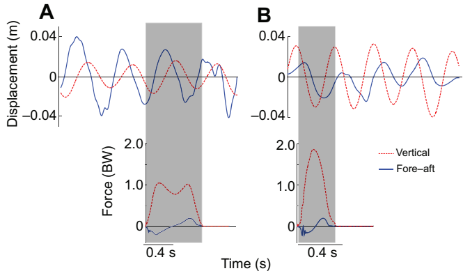
Fig. 2. Lab-based measures of fore–aft and vertical displacement with synchronized ground reaction forces, as validation of the gait detection technique used for the GPS-IMU logger data. (A) Walking at relative speed V =0.38 (1.34 m s -1 ). (B) Running at V =0.75 (2.64 m s -1 ). The displacements were calculated from kinematics of a marker placed on the back of the ostrich above the position of the centre of mass (CoM) in the dorsal plane, comparable to the loggers. The ground reaction force traces for a single step are shown (BW, body weight). Grey boxes indicate the duration of stance.
