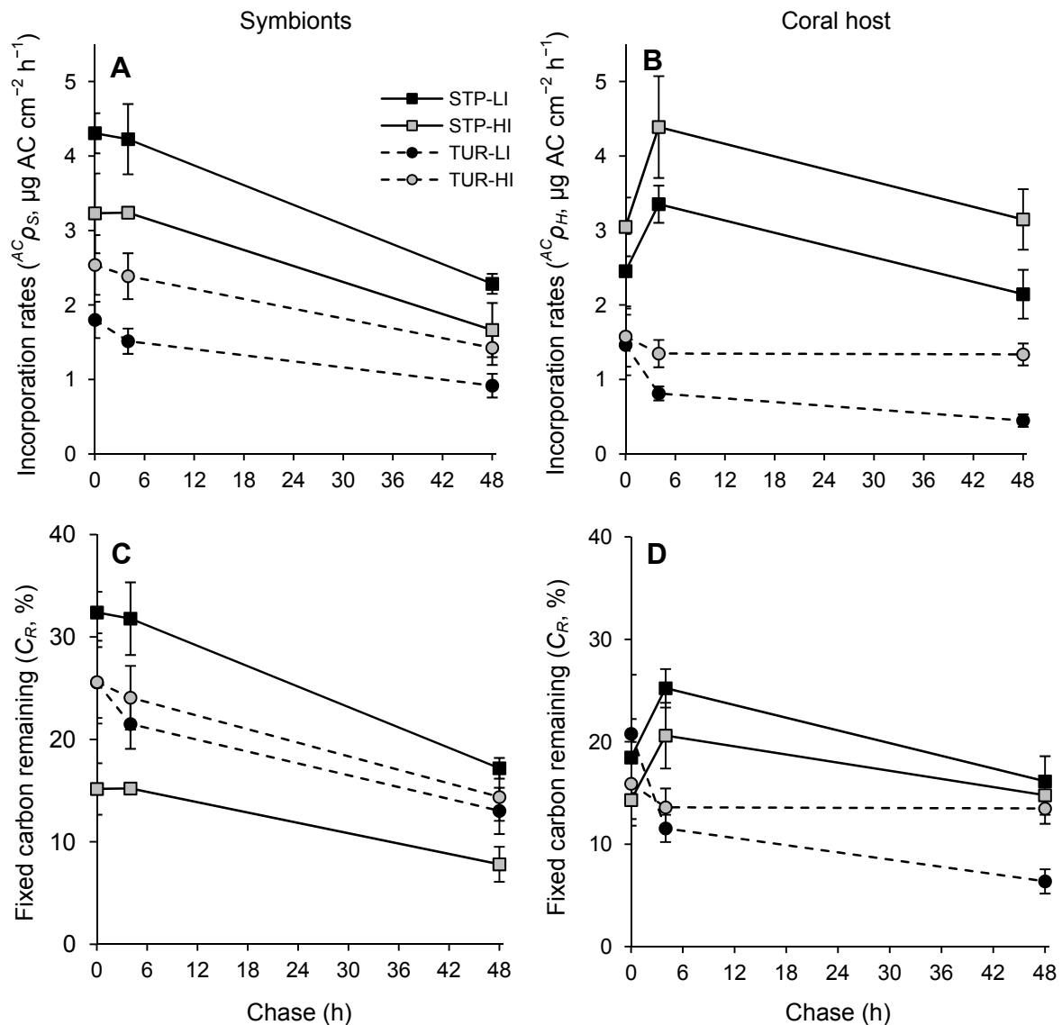
Fig. S1. Effect of species and irradiance on the autotrophic carbon (AC) incorporation rates ( ^{14}C \rho ) and percentage of fixed AC that remained ( C_R ) in symbiosis. ^{14}C \rho in (A) symbionts ( ^{14}C \rho_S ), and (B) coral host ( ^{14}C \rho_H ). C_R in (C) symbionts, and (D) coral host, for Stylophora pistillata (STP) and Turbinaria reniformis (TUR) maintained at low (LI) and high (HI) irradiance. Data are means \pm standard errors of the mean of n = 3 measurements.
