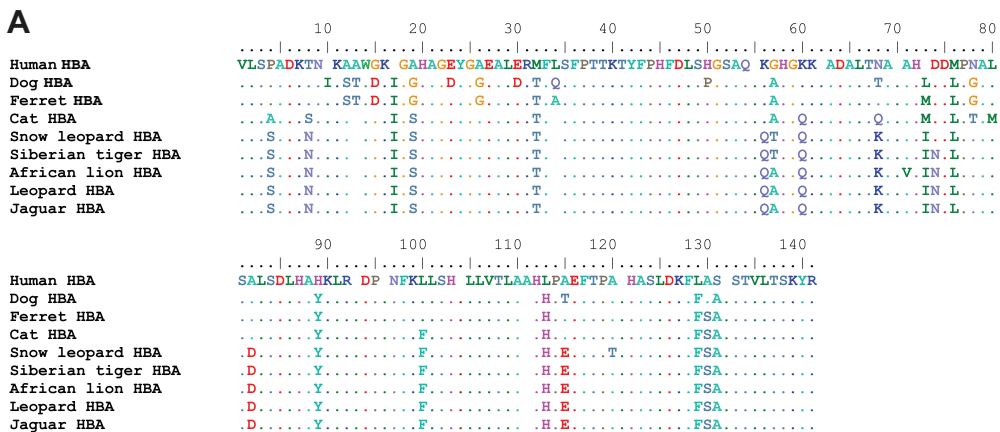
Fig. 1. Multiple sequence alignment of adult-expressed α- and β-type globins of cats and other eutherian mammals. (A) HBA α-globin genes and (B) HBB/D and HBB β-type globin genes.
