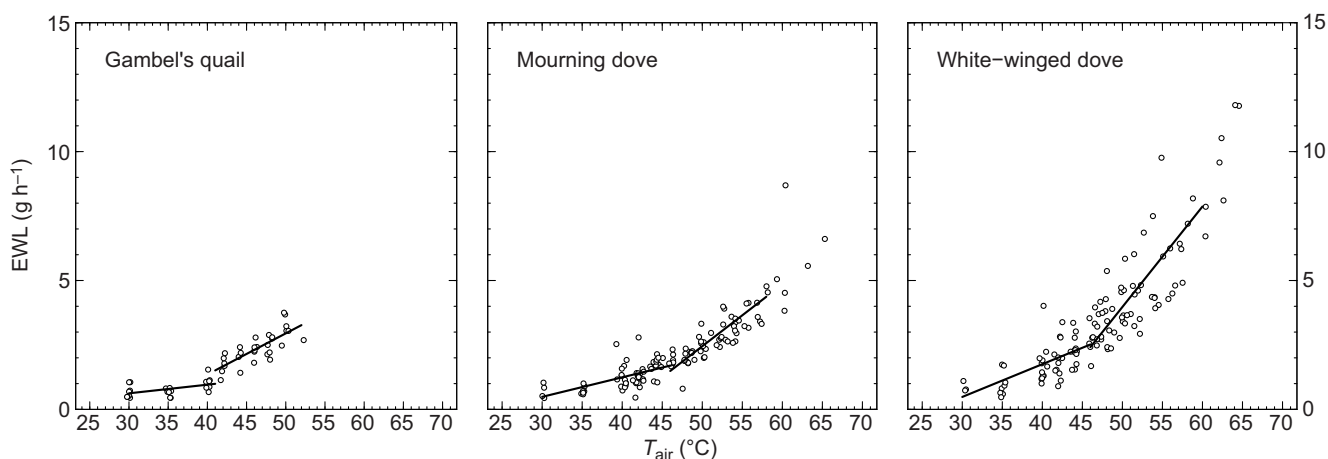
Fig. 2. Rate of evaporative water loss as a function of air temperature in Gambel's quail, mourning doves and white-winged doves. EWL was regressed against T_{\text{air}} below (all P<0.01 ) and above the T_{\text{uc}} (all P<0.001 ). T_{\text{uc}} in Gambel's quail, mourning doves and white-winged doves are 41.1, 45.9 and 46.5 ^\circ\text{C} , respectively. See text for statistical details of linear regressions, Table 2 for parameter estimates and Fig. S1 for determination of T_{\text{uc}} using RMR residuals.
