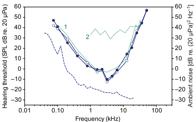
Fig. 2. Aerial audiograms for two spotted seals, Amak (filled circles) and Tunu (open circles), obtained using psychophysical methods. Ambient noise in the acoustic testing chamber is plotted as a dashed line corresponding to the right-hand y-axis. The noise profile comprises power spectral density levels [in dB re. (20 \mu Pa) 2 Hz -1 ] calculated from the median of 1/3-octave band 50th percentile levels measured across all sessions. Previously published thresholds are shown for harbor seals [1, N =1 (Reichmuth et al., 2013)] and harp seals [2, N =1 (Terhune and Ronald, 1971)]. SPL, sound pressure level.
