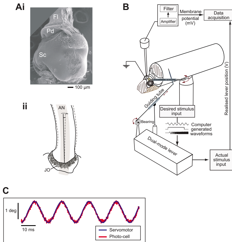
Fig. 1. Experimental set-up for intracellular recordings of the scolopial responses to antennal vibrations.
