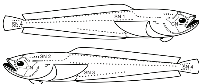
Fig. 3. Schematic illustration of the plainfin midshipman fish lateral line mechanosensory system (adapted from Greene, 1899). All illustrated neuromasts and several stitches not illustrated [superficial neuromasts (SN) primarily on the head and underbelly] were targeted for ablation. Four regions of SN were selected for phalloidin labeling (neuromasts filled in black): a 2 cm region from the right dorsal line starting at the anterior edge of the dorsal fin (SN 1), a 1 cm region on the top of the head (left side; SN 2), 1.5–2 cm from the ventral line (left side) starting at the anterior edge of the anal fin (SN 3), and the entire caudal fin (SN 4). Given the small number of canal neuromasts (CN) in this species, all canals were dissected from the head and labeled rather than selecting discrete CN regions for sub-sampling (arrows; neuromasts within canals not illustrated).
