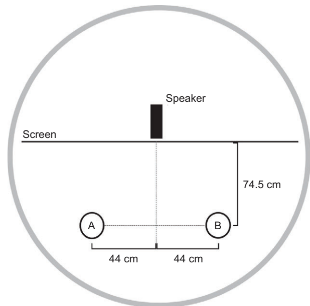
Fig. 1. Schematic of the experimental setup (tank diameter=4 m, water depth=50 cm). Shown is the monopole sound source (Lubell AQ339, Clark Synthesis, Littleton, CO, USA, or a US Navy J-9 transducer), the opaque screen and the animal release sites (A and B).
