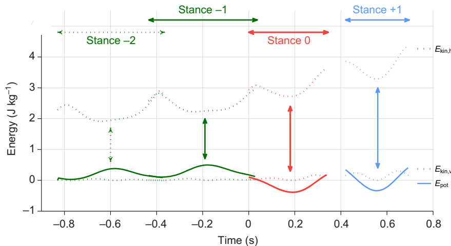
Fig. 1. Energy fluctuations of the body centre-of-mass (BCOM) during the spontaneous walk-to-run transition (WRT). Solid lines represent the potential energy ( E_{\text{pot}} ), indicating the switch from an inverted pendulum (step -2 and step -1) to a spring-mass (step 0, step +1). Upper dotted lines represent the horizontal kinetic energy ( E_{\text{kin,h}} ); lower dotted lines represent the vertical kinetic energy ( E_{\text{kin,v}} , maximum 0.33 \text{ J kg}^{-1} ). The arrows indicate the out-of-phase energy fluctuations of BCOM for step -2 and step -1 (green) and the in-phase energy organization of gravitational E_{\text{pot}} and E_{\text{kin}} for step 0 and step +1 (red and blue). Time 0 is the heel contact transition step.
