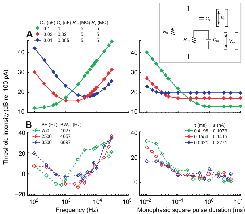
Fig. 3. Modeling the knollenorgan receptor as a simple electrical circuit. (A) Frequency (left) and duration (right) tuning curves generated from three model neurons with resistance values set to 5 M \Omega and variable capacitance values as indicated. Inset shows the electrical circuit model of knollenorgan receptors, which consists of skin resistance ( R_s ), membrane resistance ( R_m ), membrane capacitance ( C_m ) and series capacitance ( C_s ). Corresponding voltage drops ( V_s and V_m ) across the two capacitors are shown with arrows. (B) Frequency (left) and duration (right) tuning curves from three different knollenorgans recorded from a single fish with measured values for best frequency (BF), bandwidth (BW 10 ), duration tuning curve time constant ( \tau ) and duration tuning curve asymptote ( a ).
