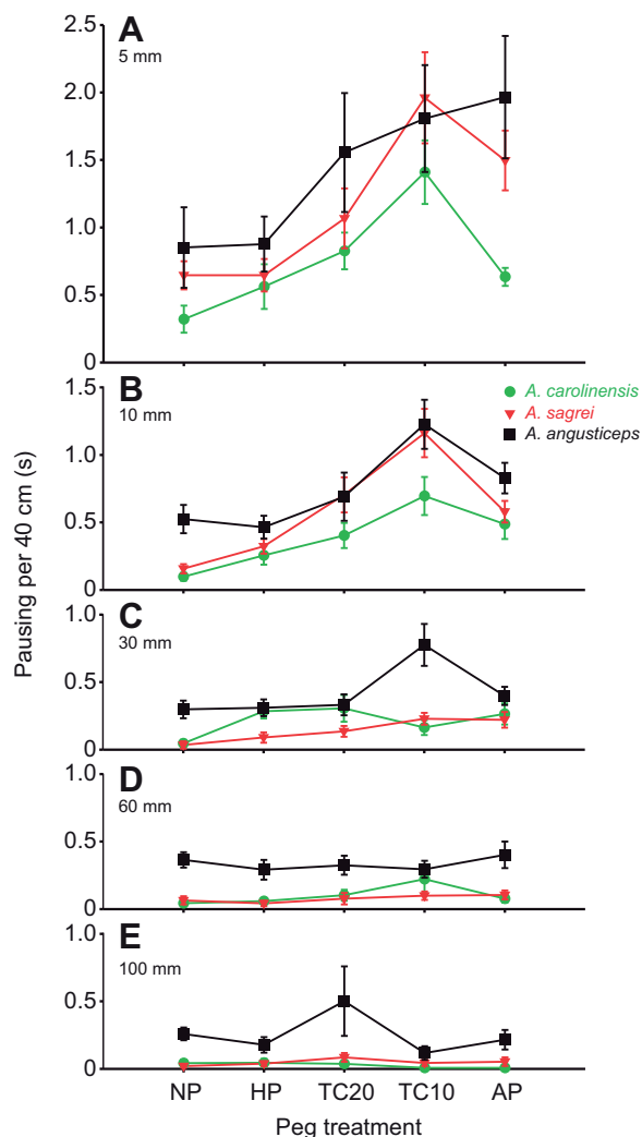
Fig. 4. Mean values of total pause duration per 40 cm, illustrating the combined effects of perch diameter and different patterns of peg placement. Abbreviations are as in Fig. 3. The addition of any pegs along the top of the perch (TC20, TC10 and AP) was most likely to increase the amount of pausing on the smaller diameters.
