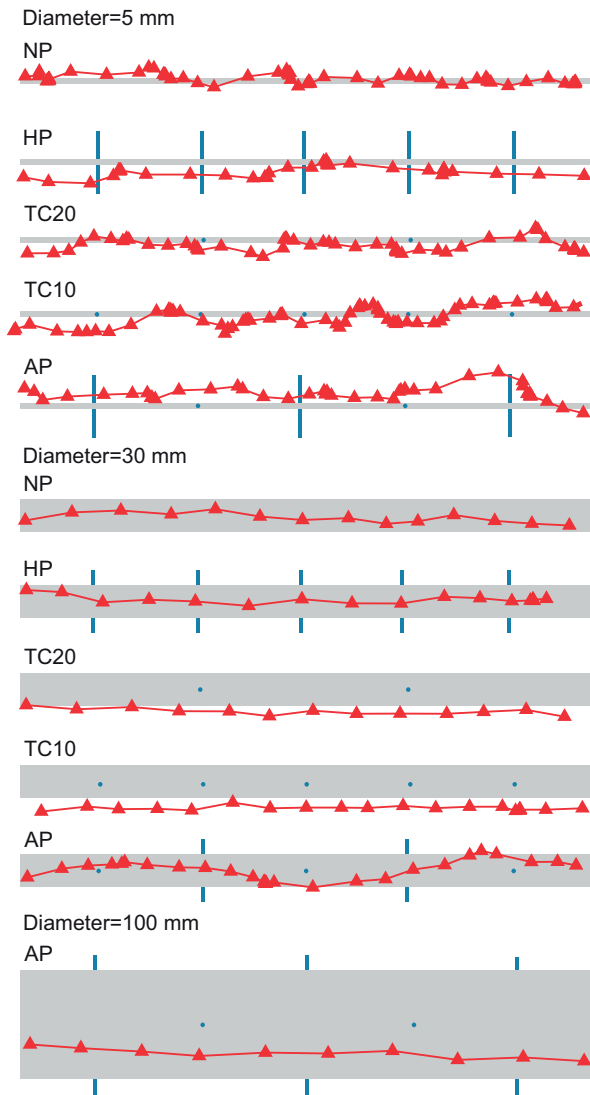
Fig. 9. Dorsal views of the position of the head of a single individual of A. sagrei running on a variety of perch diameters with different peg arrangements. Abbreviations are as in Fig. 3. The time between successive points within each panel is 40 ms. The less even spacing of points illustrates the more unsteady and intermittent movement that was common on narrower surfaces, especially when pegs were present along the top surface of the cylinder. Note the detouring behavior on the 30 mm diameter perches with pegs along the top (TC20, TC10), whereas the lizard wove its way through the pegs along the top of the 30 mm diameter perch with alternating pegs (AP).
