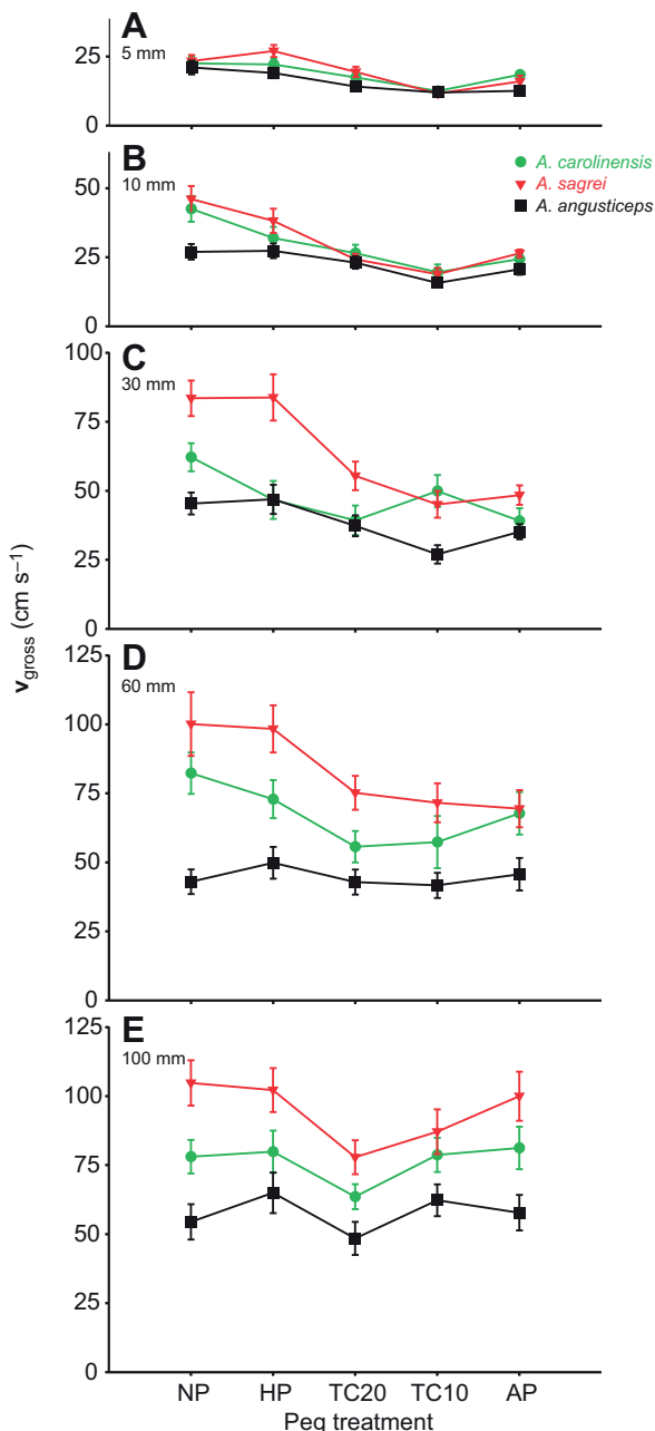
Fig. 3. Mean values of performance illustrating the combined effects of perch diameter and different locations of pegs. NP, no pegs were present; HP and AP, pairs of pegs were present every 10 cm and were oriented only in a horizontal plane or alternately in a horizontal plane and then a vertical plane, respectively; TC10 and TC20, pegs were present along the top center of the cylinder spaced at 10 or 20 cm intervals, respectively. The most conspicuous effects of pegs on performance usually occurred for the intermediate cylinder diameters, but magnitude of the effects of pegs also depended upon the species.
