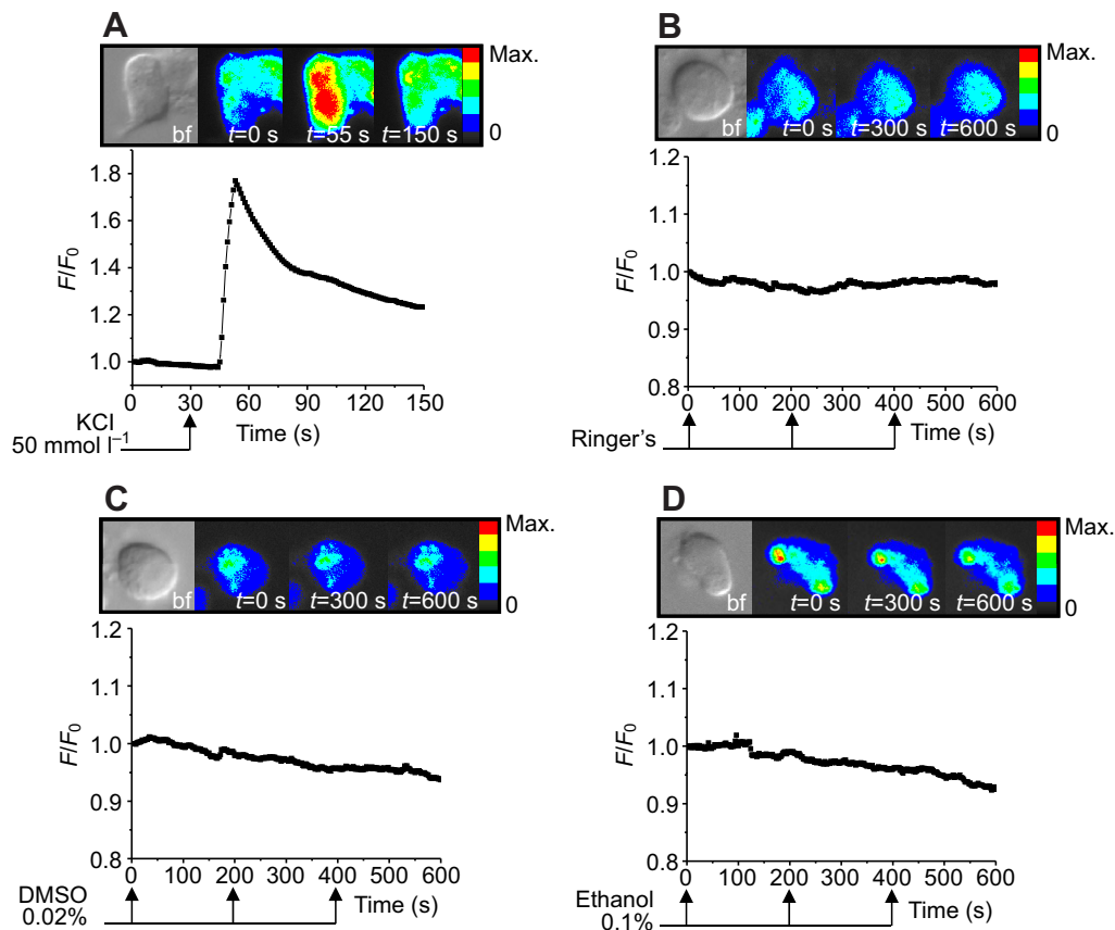
Fig. 2. Controls used in the odorant analysis in rainbow trout. (A) Depolarization of crypt cells with 50 \text{ mmol l}^{-1} KCl triggered large and reversible calcium signals ( F/F_0 ), and was used as positive control ( N=20 cells from three fish). Fluorescence images show calcium signals before, during and after the stimulus. Color scales indicate relative fluorescence intensity. (B–D) Stimulation with pure Ringer's solution ( N=181 cells from 15 fish) or the solvents DMSO and ethanol ( N=15 cells from three fish each) at the concentration used for odorant dilution did not elicit significant calcium signals in any tested cell.
