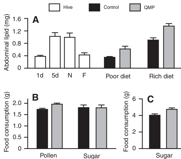
Fig. 5. Effects of queen mandibular pheromone (QMP) on abdominal lipid stores and food consumption. (A) Abdominal lipid stores of hive-reared 1 day old bees (1d), 5 day old bees (5d), nurses (N) and foragers (F), and of cage-reared 5 day old bees fed either rich or poor diet in combination with exposure to QMP or a solvent control. Means + s.e.m. N=30 bees. ANOVA for diet \times QMP factorial: P_{\text{diet}}=1.0e-8 , P_{\text{QMP}}=0.006 , P_{\text{diet}\times\text{QMP}}=0.20 . (B) Effects of QMP on food consumption (total consumption over 4 days for cages containing 35 bees) by bees fed a rich diet of both pollen paste and sugar syrup and exposed to either QMP or a solvent control. N=6 cages. (C) Effects of QMP on food consumption by bees fed a poor diet of sugar syrup only. N=8 cages. In B and C, bars indicate least square means and their standard errors based on ANOVA for QMP exposure and trial. * P_{\text{QMP}}<0.05 .
