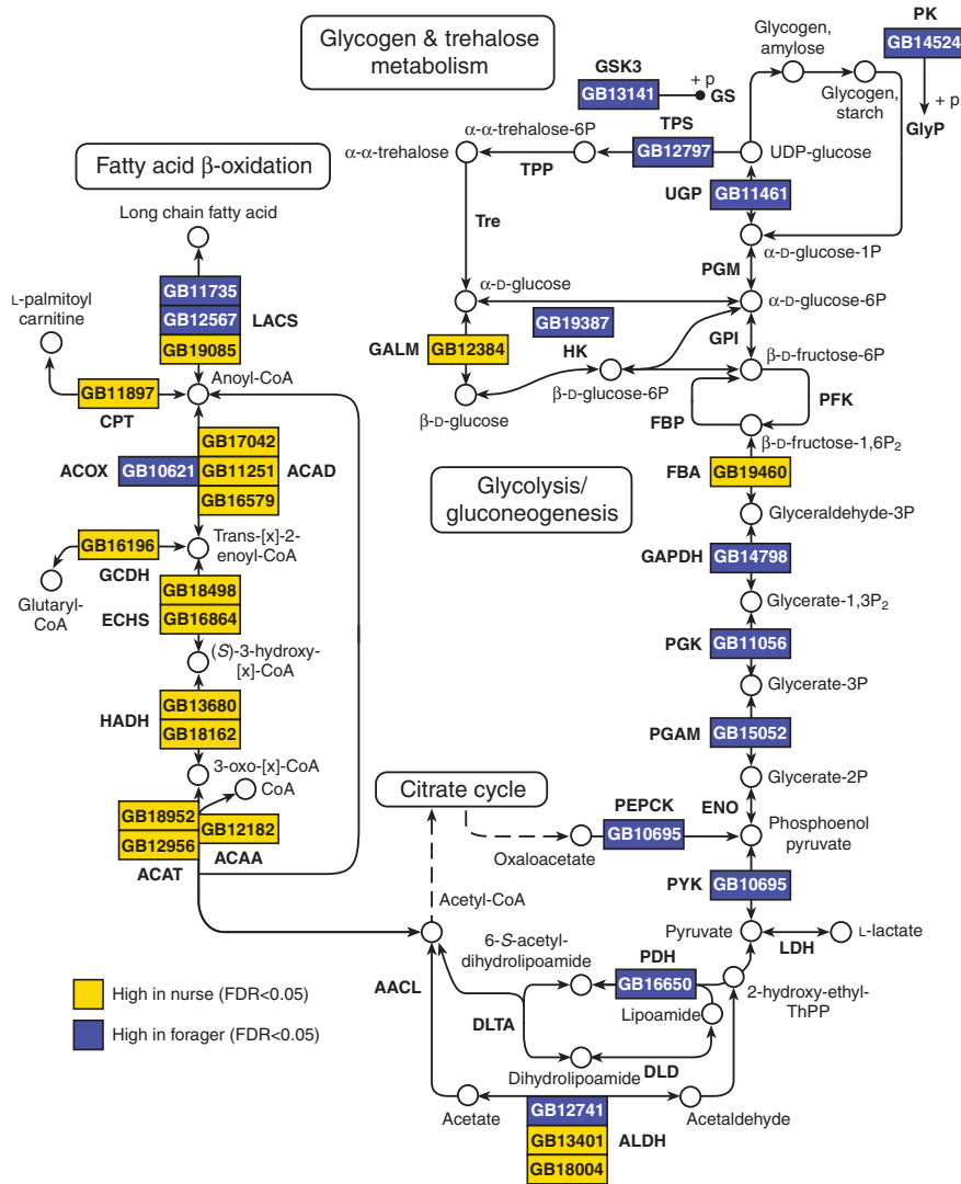
Fig. 1. Maturation changes in fatty acid and carbohydrate metabolism gene expression. Transcripts differentially expressed between nurse and forager fat bodies (false discovery rate, FDR < 0.05 ) were mapped to metabolic pathways based on the union of direct annotations from the Kyoto Encyclopedia of Genes and Genomes (KEGG) and the KEGG annotations for Drosophila orthologs of honey bee genes. Pathway diagrams are modified from portions of KEGG maps for glycolysis/gluconeogenesis (00010), starch and sucrose metabolism (00500), and fatty acid metabolism (00071).
