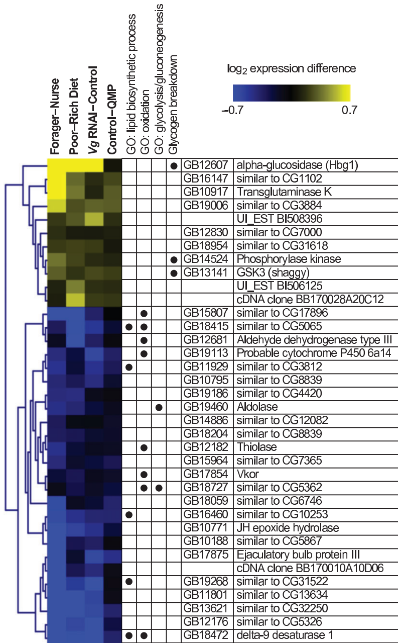
Fig. 6. Genes with concordant responses to maturation, diet, vg RNAi and QMP. Genes are shown that responded significantly (FDR<0.2) in all four experiments in concordant directions relative to the effects of each factor on a bee's lipid stores. Heatmap shows the log 2 transformed difference estimate in each experiment. Dots indicate annotation of a gene to the GO biological processes listed or manually annotated to glycogen breakdown. Gene names are listed according to the A. mellifera Official Gene Set 2 (Honeybee Genome Sequencing Consortium, 2006) and their orthology to Drosophila melanogaster genes based on Reciprocal Squared Distance or reciprocal BLAST. Oligos corresponding to unannotated ESTs are listed according to the EST name.
